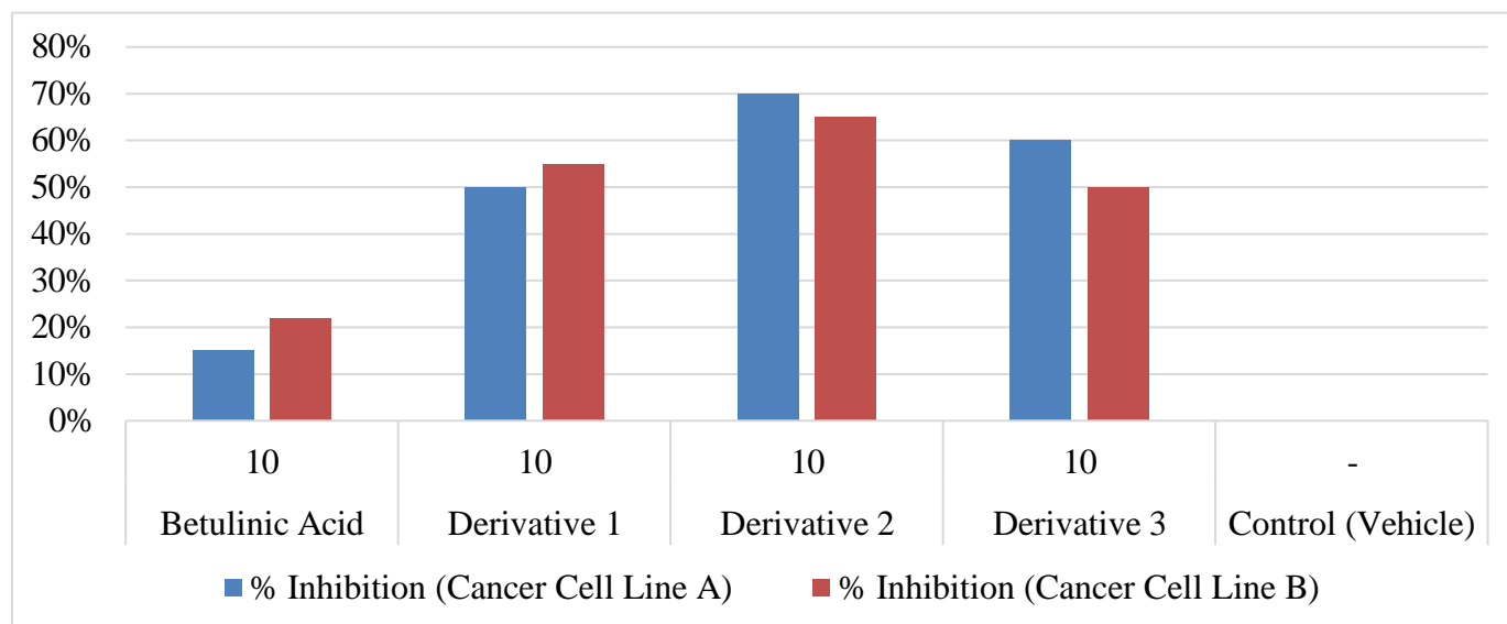
Figure 3: Graphical Presentation of Percentage of Cancer Cell Survival Following Betulinic Acid Derivative Therapy
