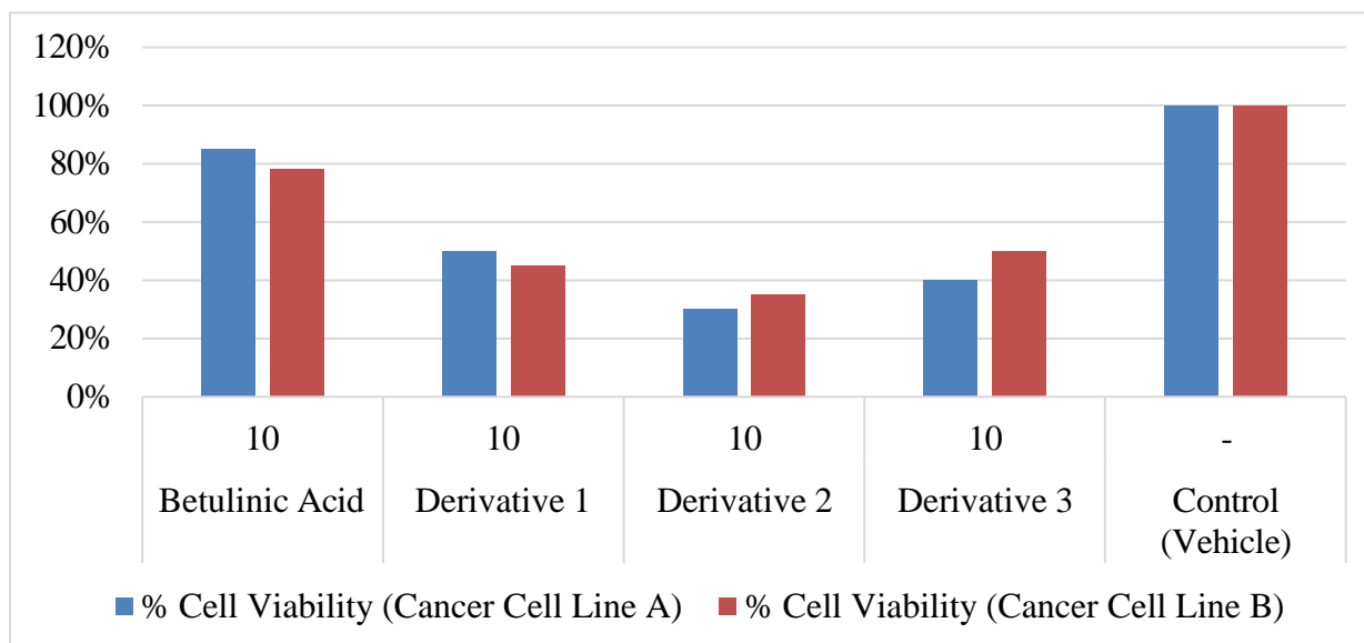
Figure 1: Percentage of Cancer Cell Survival Following Betulinic Acid Derivative Therapy
